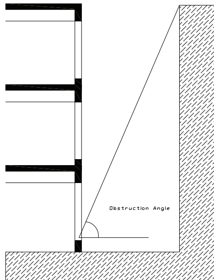
Figure No.1 – Angle of Obstruction
